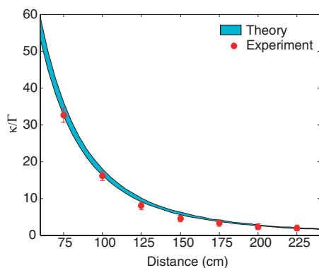
Fig. 3. Comparison of experimental and theoretical values for the parameter \kappa/\Gamma as a function of the wireless power transfer distance. The theory values are obtained by using the theoretical \kappa and the experimentally measured \Gamma . The shaded area represents the spread in the theoretical \kappa/\Gamma due to the 5% uncertainty in Q .
