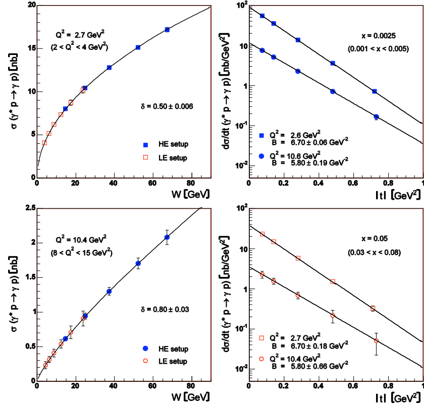
Figure 8. (a) Left panel: projected results for the total DVCS cross section with an EIC, as a function of W for two values of Q^2 . (b) Right panel: differential cross section ds/dt for two representative values of x and Q^2 . The projections assume a high-energy setup (10 on 250 GeV), with an integrated luminosity of 530 \text{ pb}^{-1} for the smaller x -value, and a low-energy setup (5 on 50 GeV) with 180 \text{ pb}^{-1} for the larger x -value. The estimates of the event rates here assume 100% detector acceptance.
