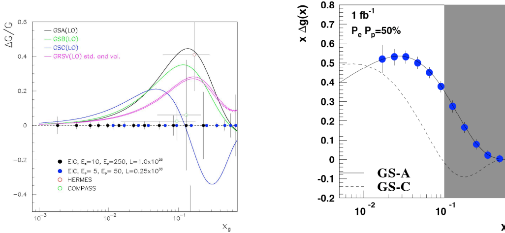
Figure 7. (a) Left: projected uncertainties in the determination of \Delta g(x)/g(x) at EIC using the channel D^0 - K^+\pi^- in charm production. The integrated luminosity is 10 \text{ fb}^{-1} for the 10 GeV electron on 250 GeV proton measurement, and 2.5 \text{ fb}^{-1} for 5 GeV electrons on 50 GeV protons. We also show the currently available COMPASS and HERMES data points on \Delta g(x)/g(x) from the photon-gluon fusion process. (b) Right: expected statistical uncertainties of the extracted spin-dependent gluon distribution from measurements of ep \rightarrow \text{jet jet } X at EIC, assuming 1 \text{ fb}^{-1} luminosity[21].
