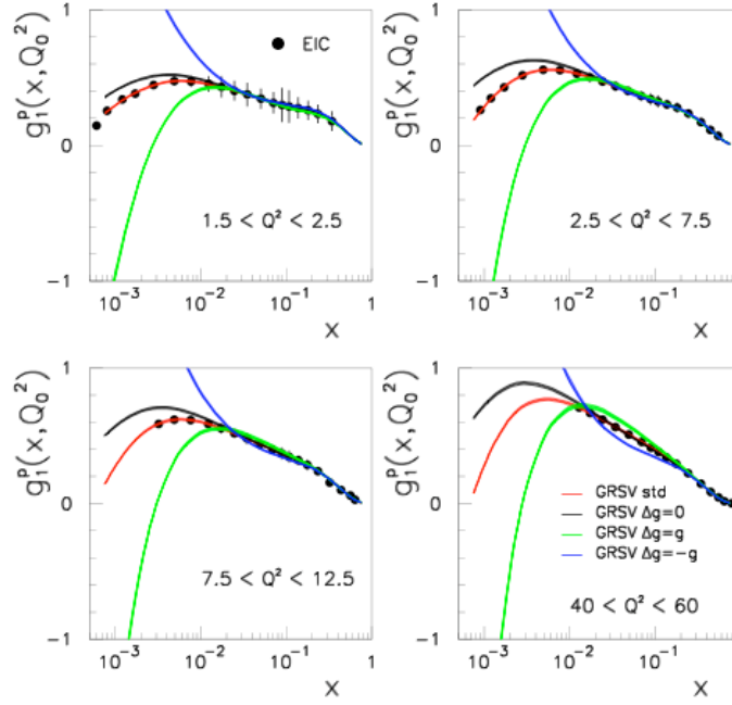
Figure 6. Projected EIC data for the proton structure function g_1(x, \mathcal{Q}^2) as a function of x in four \mathcal{Q}^2 bins, measured in 150 \text{ GeV} \times 7 \text{ GeV} collisions, for 5 \text{ fb}^{-1} integrated luminosity. Error bars are statistical. The curves show the theoretical predictions based on different sets of spin-dependent parton distribution functions of [20].
